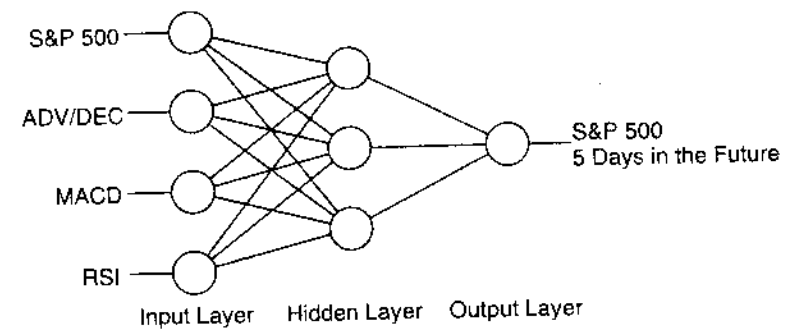
Figure 9-3 Simple three-layer artificial neural network for predicting the S&P 500 five days in advance using today's value of the S&P 500, the Advance/Decline Index, MACD, and RSI as inputs.
