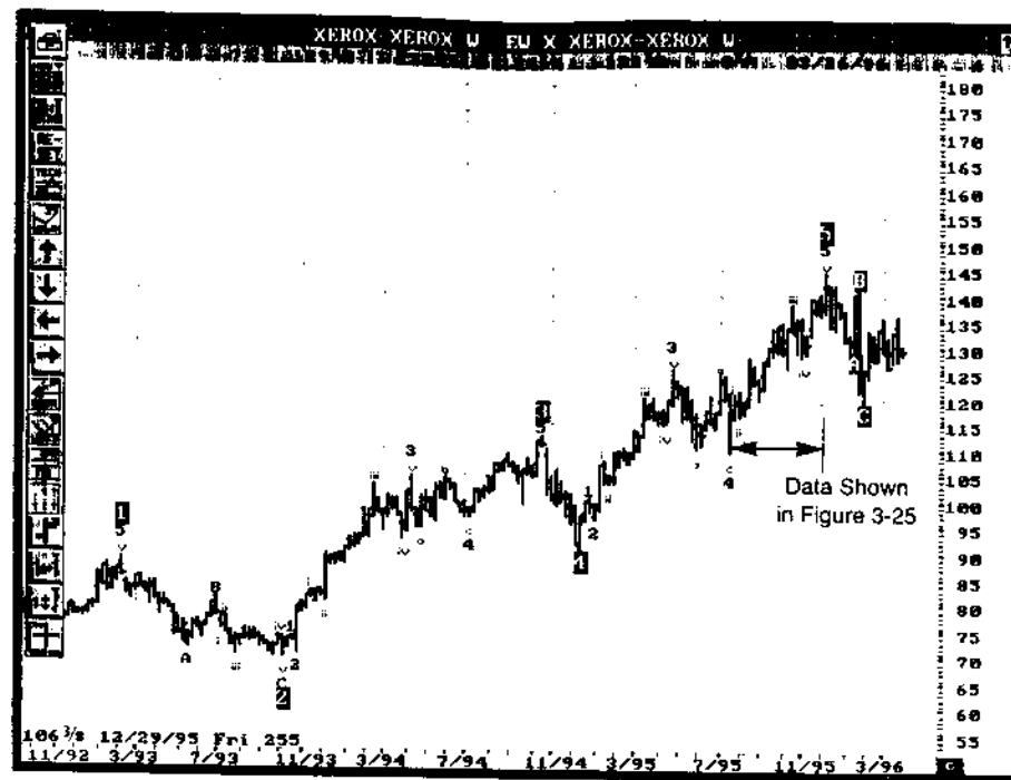
Figure 3-27 Weekly chart of Xerox. Note the information shown in Figure 3-25 occupies only a small section of this chart. This shows that Elliott waves can be applied in all time frames.
